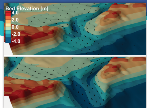
Morphology - River Mouth Scour
