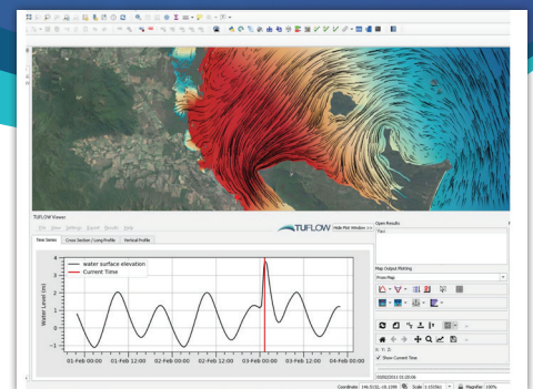
Storm Tide Result Visualization
