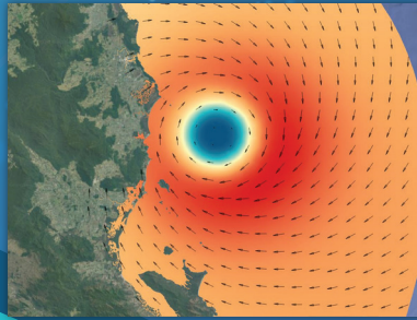
Tropical Cyclone Wind Field
