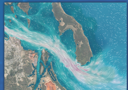
Velocity Tracers and Magnitude
