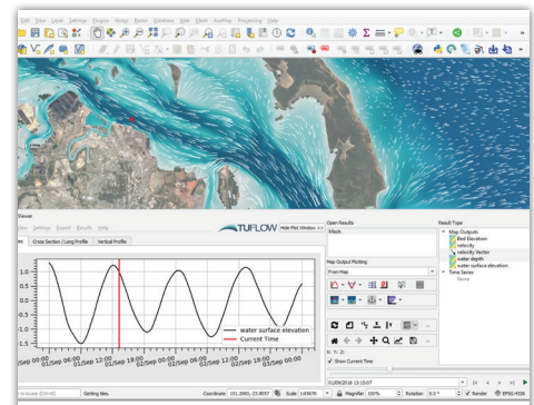
TUFLOW Viewer QGIS Plugin
