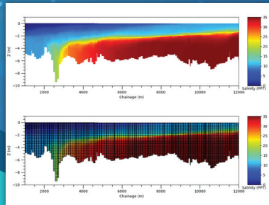
3D Salinity Output - Salt Wedge
