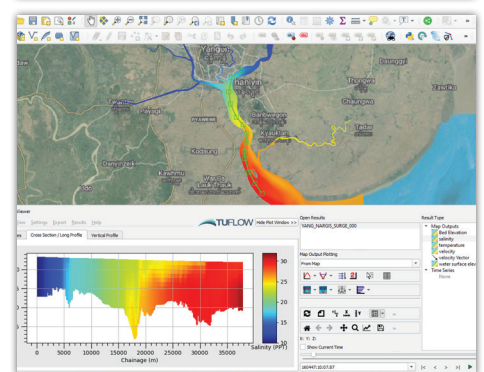
Complex estuary easily resolved with flexible mesh
